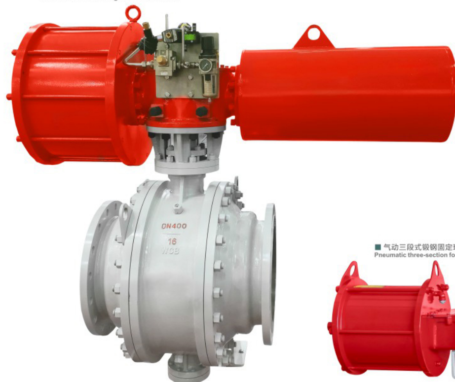
■ 气动三段式固定球阀 Pneumatic three-stage fixed ball valve
